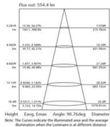
Beam diagram
